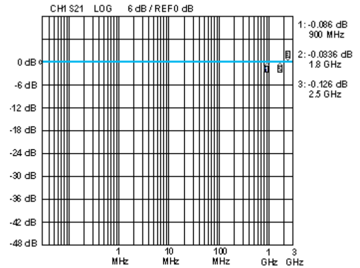
START: 0.030 MHz STOP: 3000.000000 MHz Fig. 4 Insertion Loss S21 - I/O to I/O
